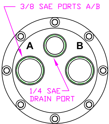
VIEW A - A
